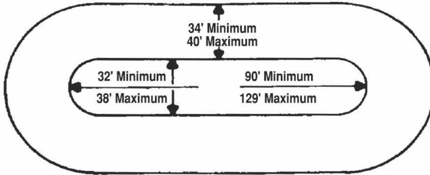
Figure 1: Track Dimension Detail
